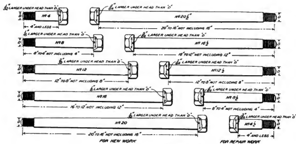
Figs. 4721-4730. Standard Taper Bolts.
